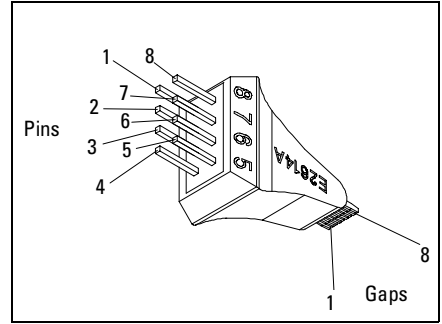
8-signal HP Wedge Probe Adapter
