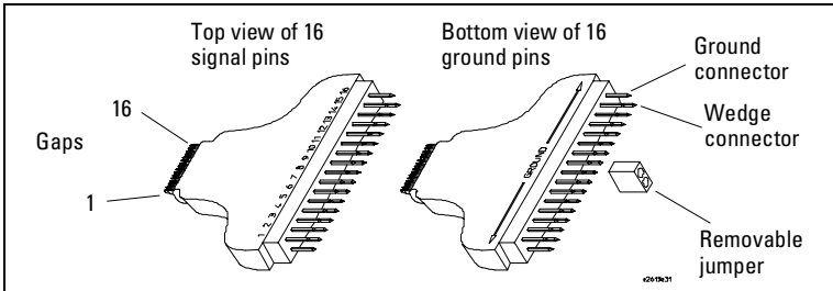
16-signal HP Wedge Probe Adapter
